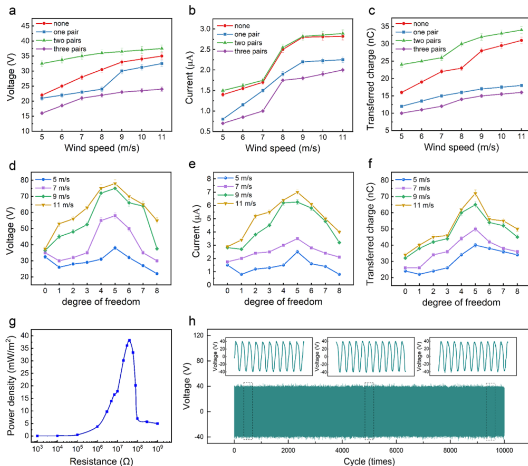
Figure 3. Electrical output performance of the HF-TENG under different pair numbers of supporting sponge strips and degrees of freedom. (a) V_{oc} , (b) I_{sc} , and (c) Q_{sc} of the HF-TENG under various wind speeds when the pair number of supporting sponge strips is 0, 1, 2, 3. (d) V_{oc} , (e) I_{sc} , and (f) Q_{sc} of the HF-TENG with different degrees of freedom. (g) Dependence of the peak power density on the loading resistances of the HF-TENG. (h) Electrical output stability of the HF-TENG.
